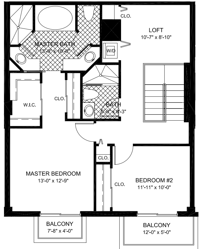
SECOND FLOOR
