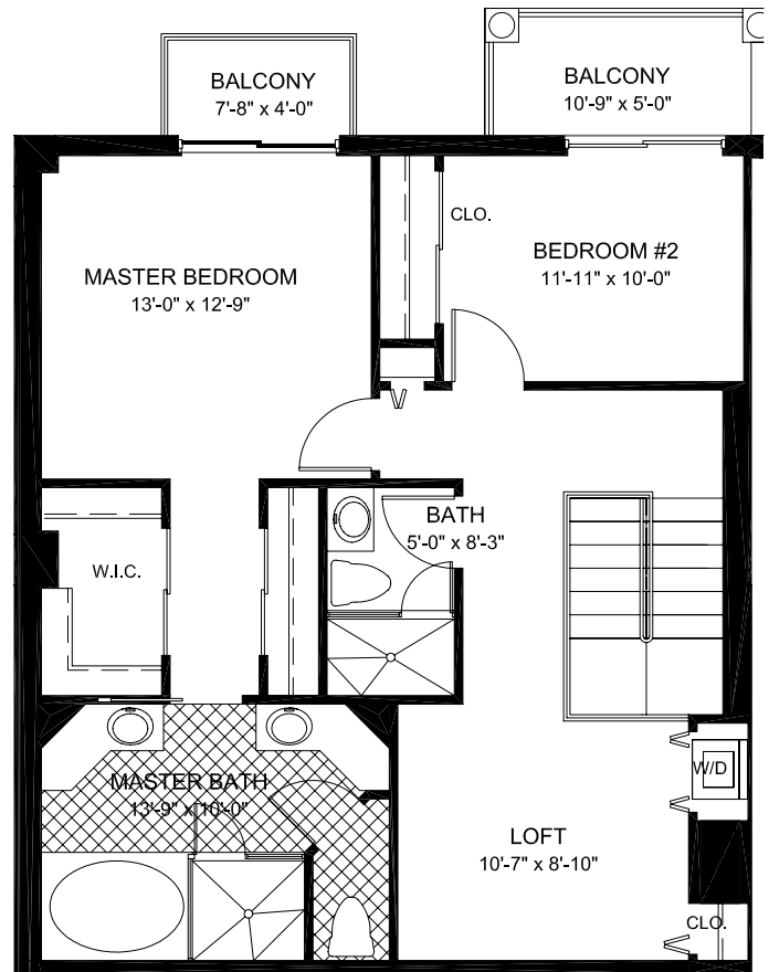
SECOND FLOOR
